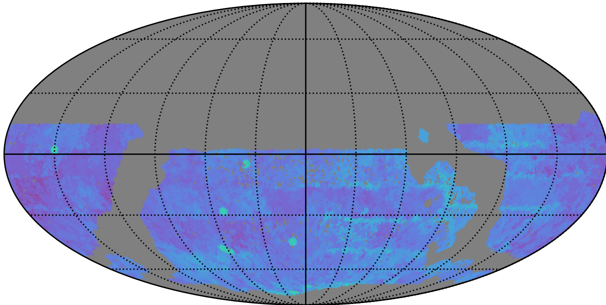
mw_roll_bulge_v3.3_10yrs WFD g band: 80thPercentile Season Length
