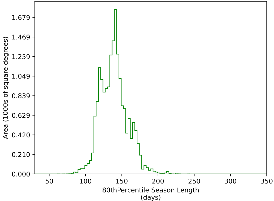
mw_roll_bulge_v3.3_10yrs WFD g band: 80thPercentile Season Length
