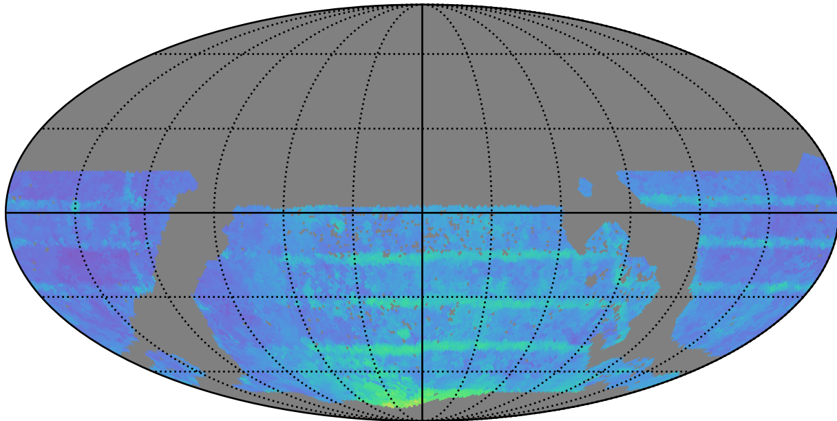
mw_roll_bulge_v3.3_10yrs WFD all bands: 80thPercentile Season Length
