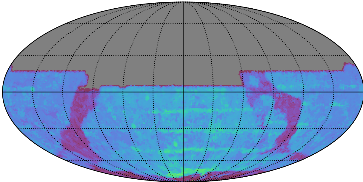
mw_roll_bulge_v3.3_10yrs All sky y band: 80thPercentile Season Length
