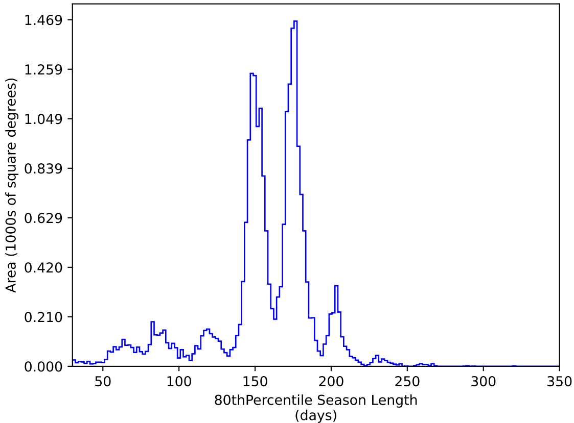
mw_roll_bulge_v3.3_10yrs All sky y band: 80thPercentile Season Length
