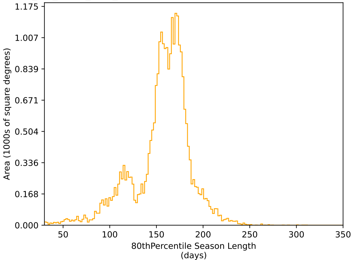
mw_roll_bulge_v3.3_10yrs All sky r band: 80thPercentile Season Length
