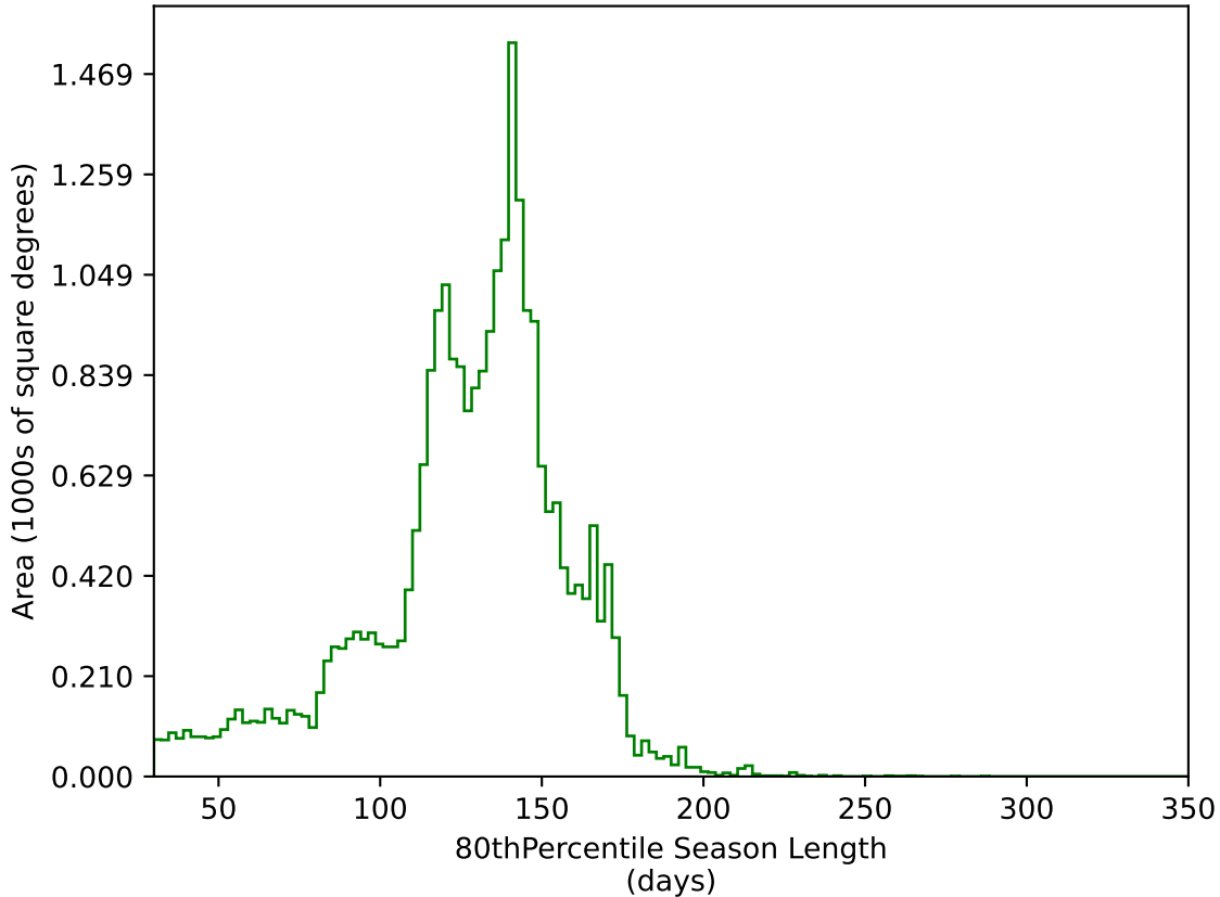
mw_roll_bulge_v3.3_10yrs All sky g band: 80thPercentile Season Length
