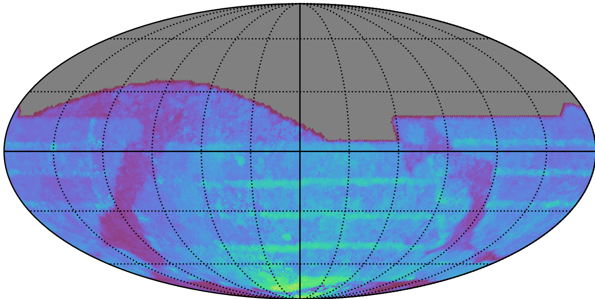
mw_roll_bulge_v3.3_10yrs All sky all bands: 80thPercentile Season Length
