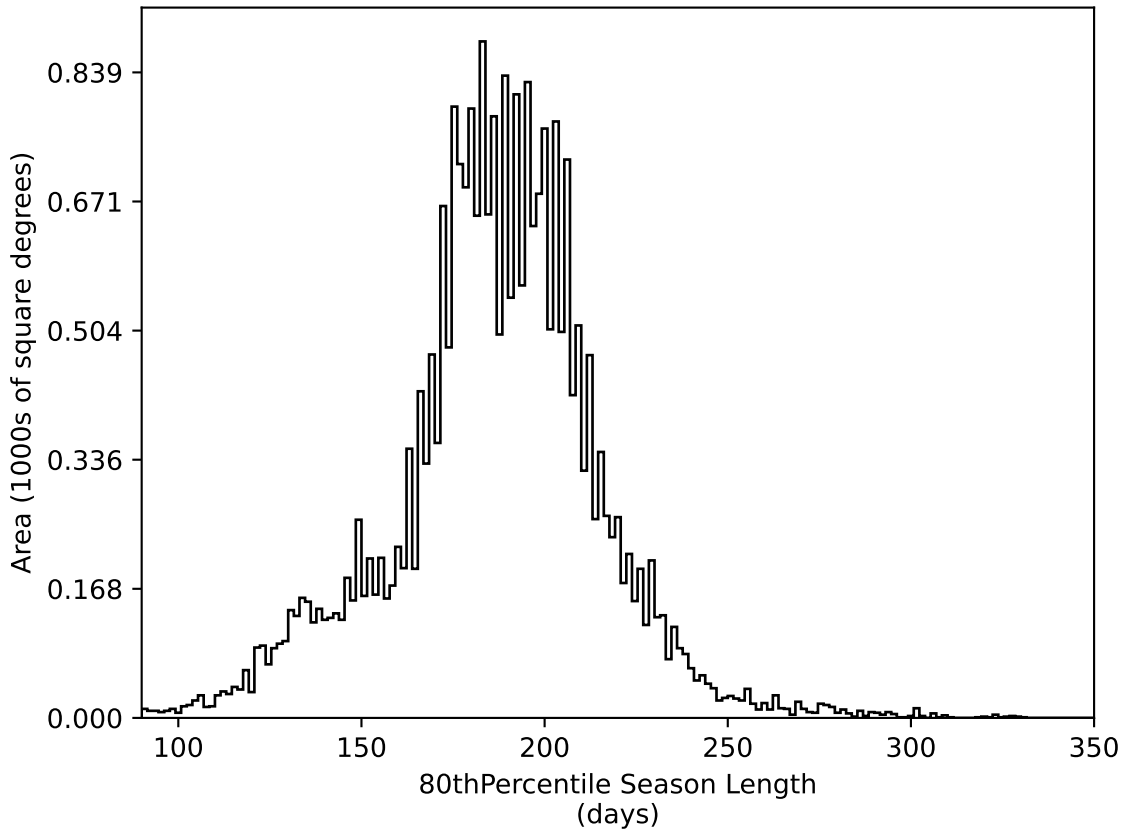
mw_roll_bulge_v3.3_10yrs All sky all bands: 80thPercentile Season Length
