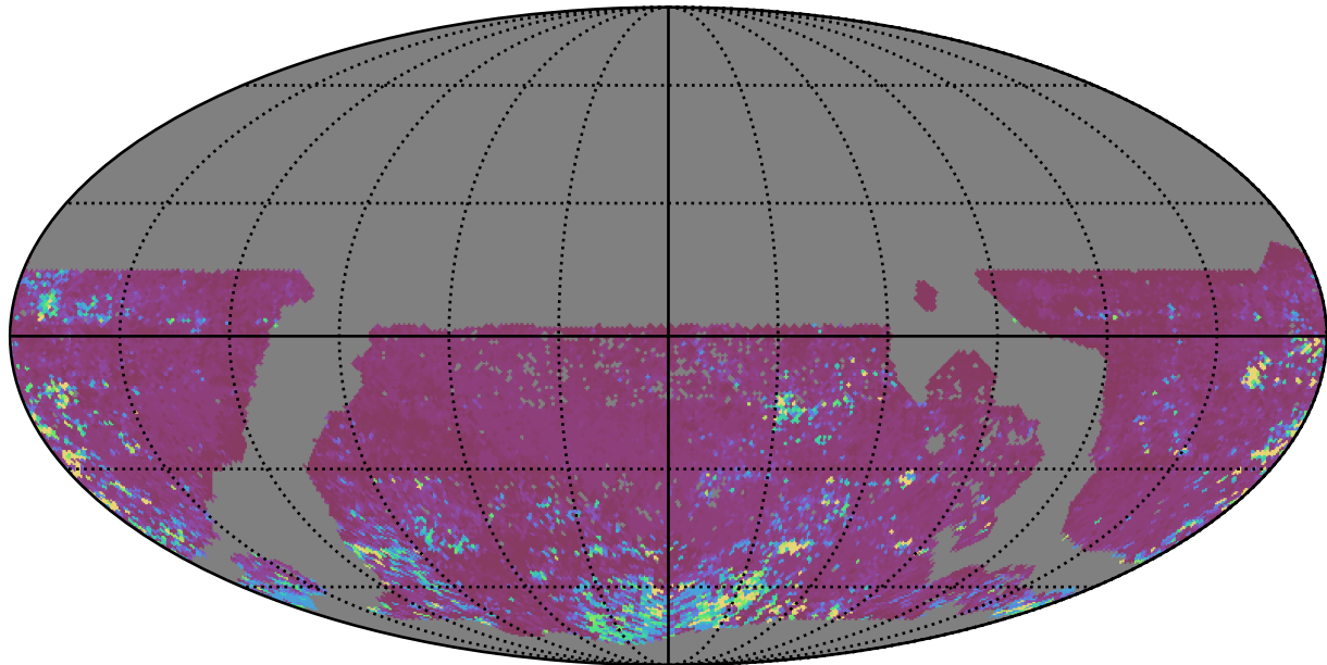
mw_roll_bulge_v3.3_10yrs WFD z band: 75th Percentile Intranight Timespan
