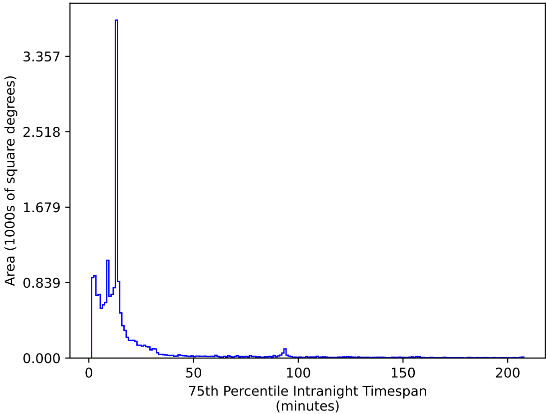
mw_roll_bulge_v3.3_10yrs WFD z band: 75th Percentile Intranight Timespan
