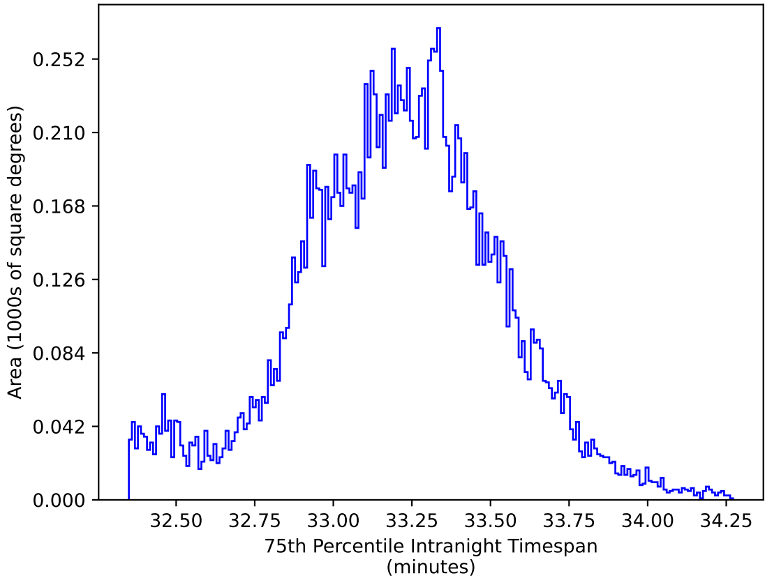
mw_roll_bulge_v3.3_10yrs WFD y band: 75th Percentile Intranight Timespan
