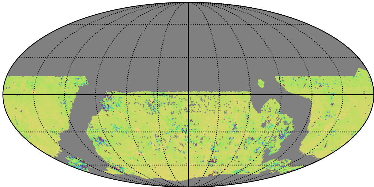
mw_roll_bulge_v3.3_10yrs WFD ug bands: 75th Percentile Intranight Timespan
