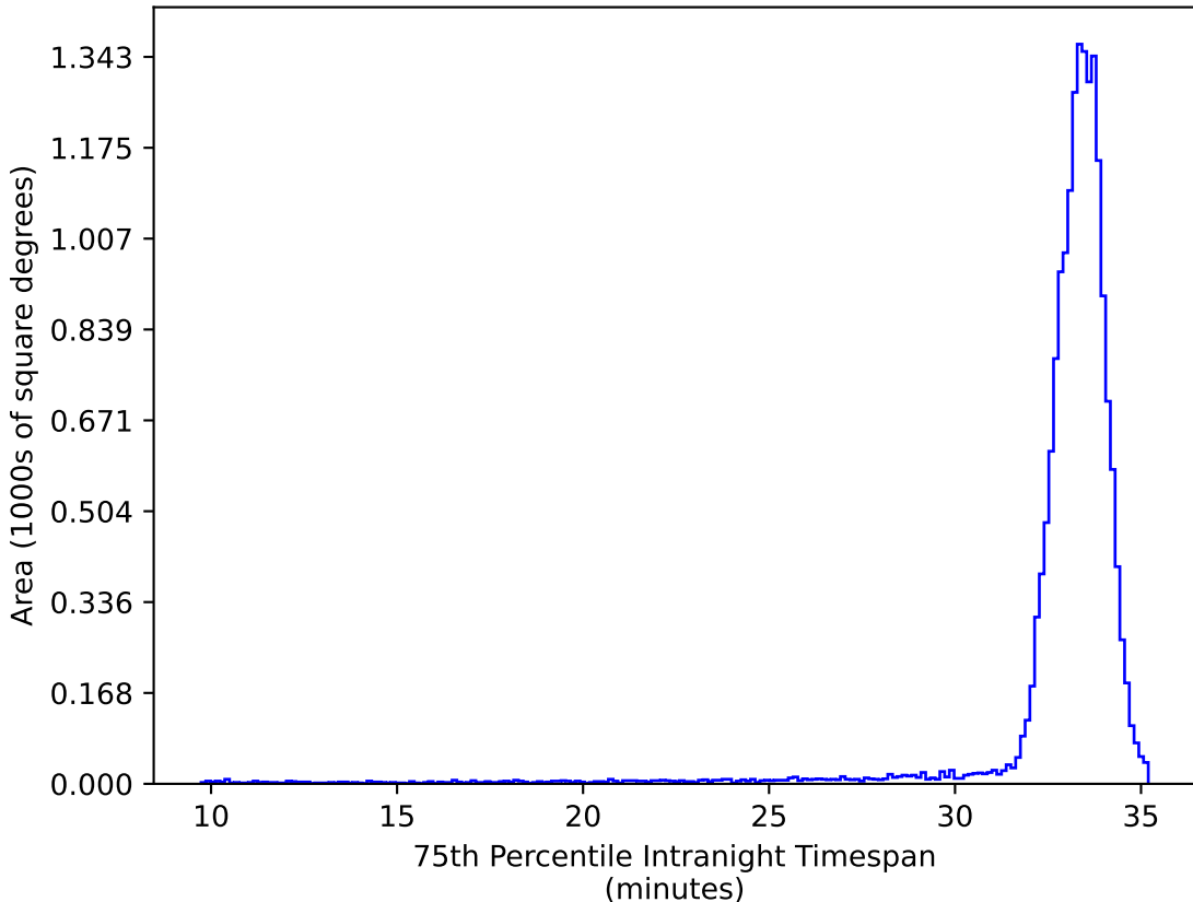
mw_roll_bulge_v3.3_10yrs WFD ug bands: 75th Percentile Intranight Timespan
