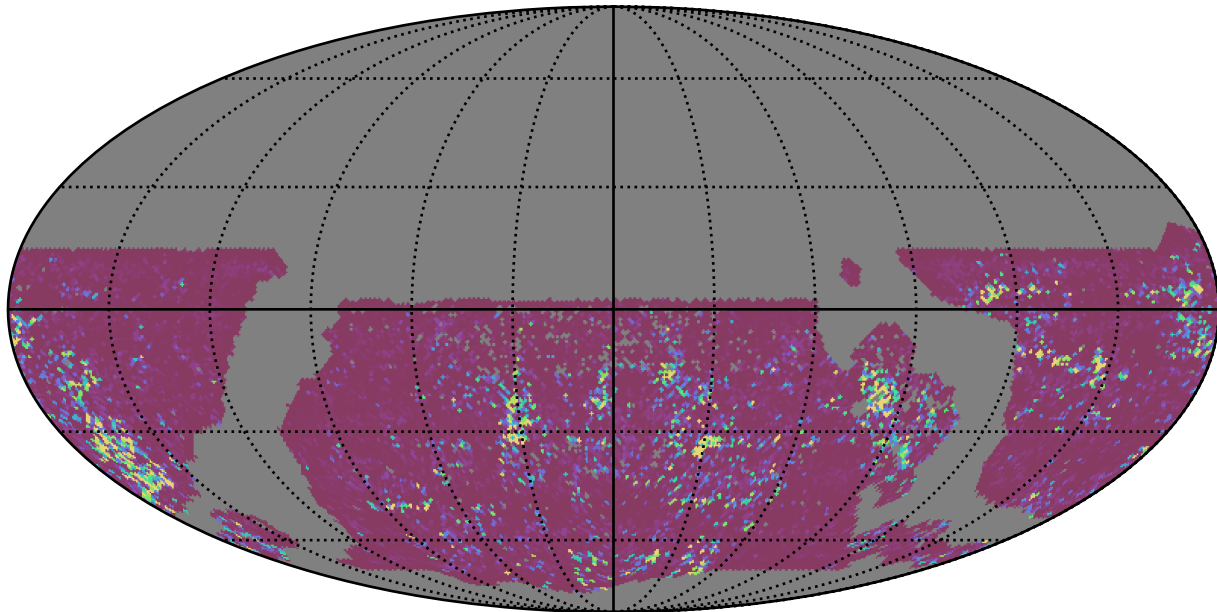
mw_roll_bulge_v3.3_10yrs WFD u band: 75th Percentile Intranight Timespan
