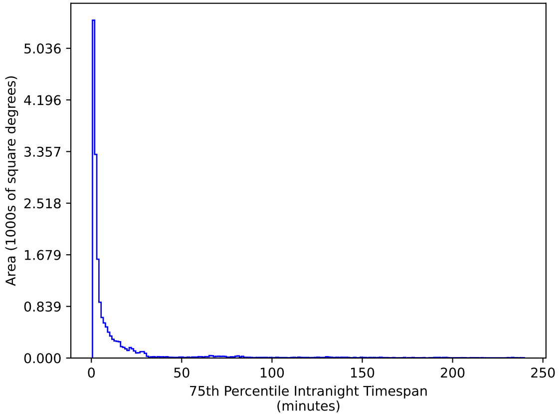
mw_roll_bulge_v3.3_10yrs WFD u band: 75th Percentile Intranight Timespan
