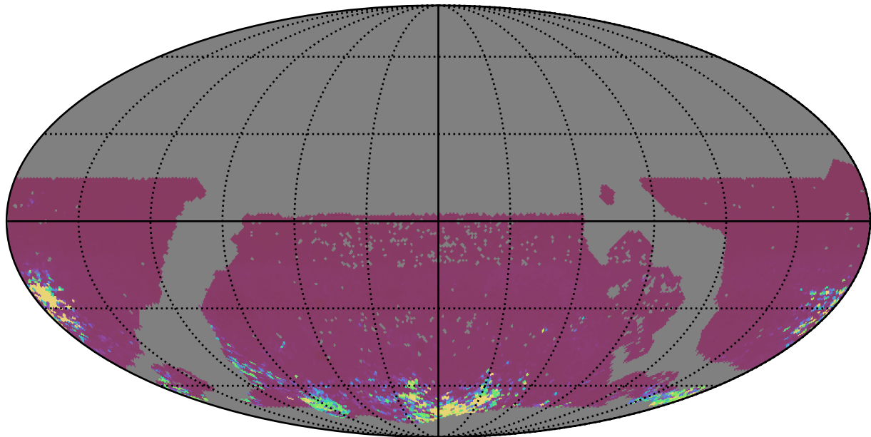
mw_roll_bulge_v3.3_10yrs WFD ri bands: 75th Percentile Intranight Timespan
