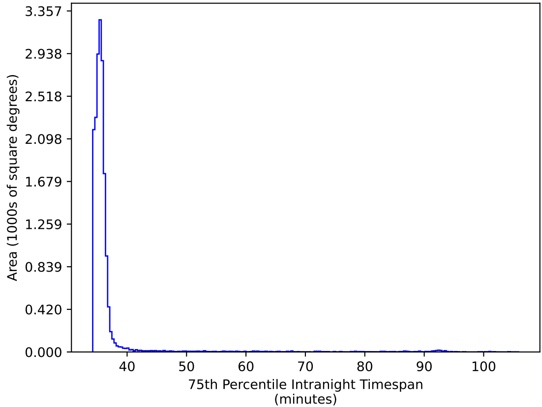
mw_roll_bulge_v3.3_10yrs WFD ri bands: 75th Percentile Intranight Timespan
