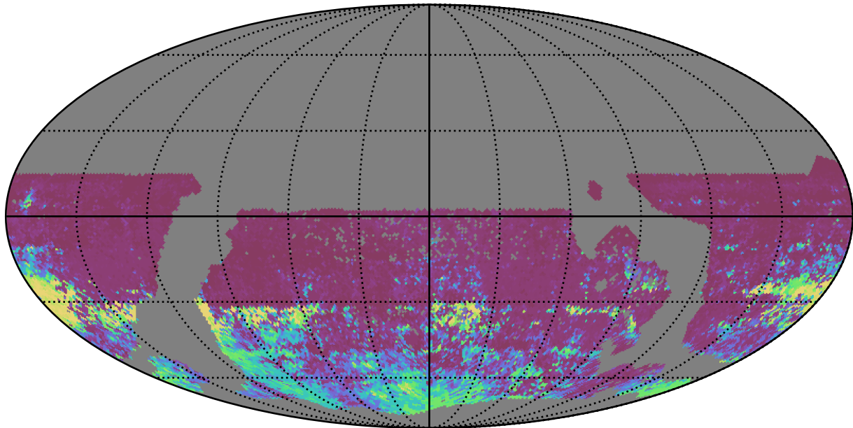
mw_roll_bulge_v3.3_10yrs WFD r band: 75th Percentile Intranight Timespan
