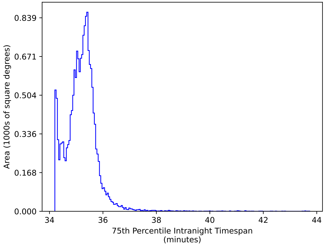
mw_roll_bulge_v3.3_10yrs WFD iz bands: 75th Percentile Intranight Timespan
