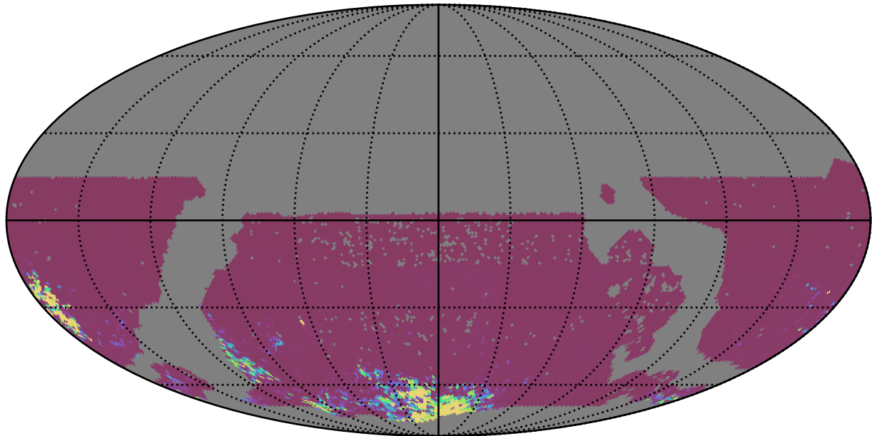
mw_roll_bulge_v3.3_10yrs WFD gr bands: 75th Percentile Intranight Timespan
