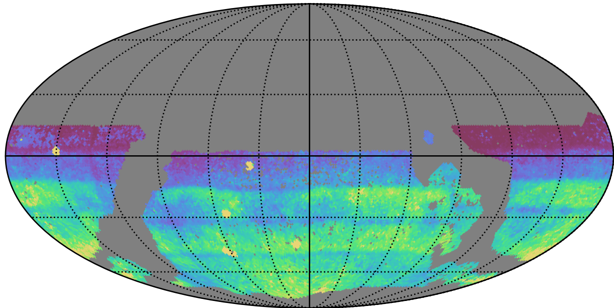
mw_roll_bulge_v3.3_10yrs WFD all bands: 75th Percentile Intranight Timespan
