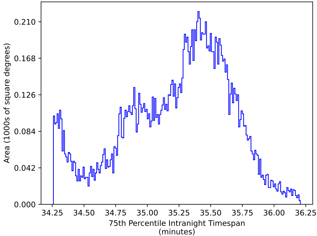
mw_roll_bulge_v3.3_10yrs WFD all bands: 75th Percentile Intranight Timespan
