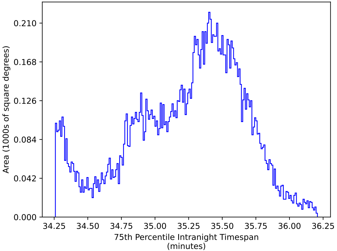
mw_roll_bulge_v3.3_10yrs WFD: 75th Percentile Intranight Timespan
