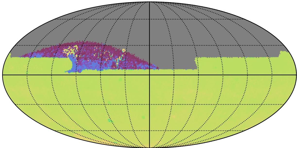
mw_roll_bulge_v3.3_10yrs All sky zy bands: 75th Percentile Intranight Timespan
