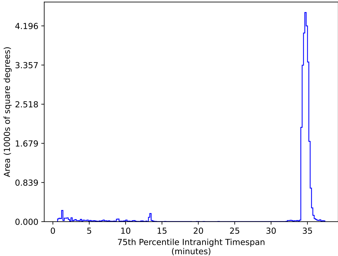
mw_roll_bulge_v3.3_10yrs All sky zy bands: 75th Percentile Intranight Timespan
