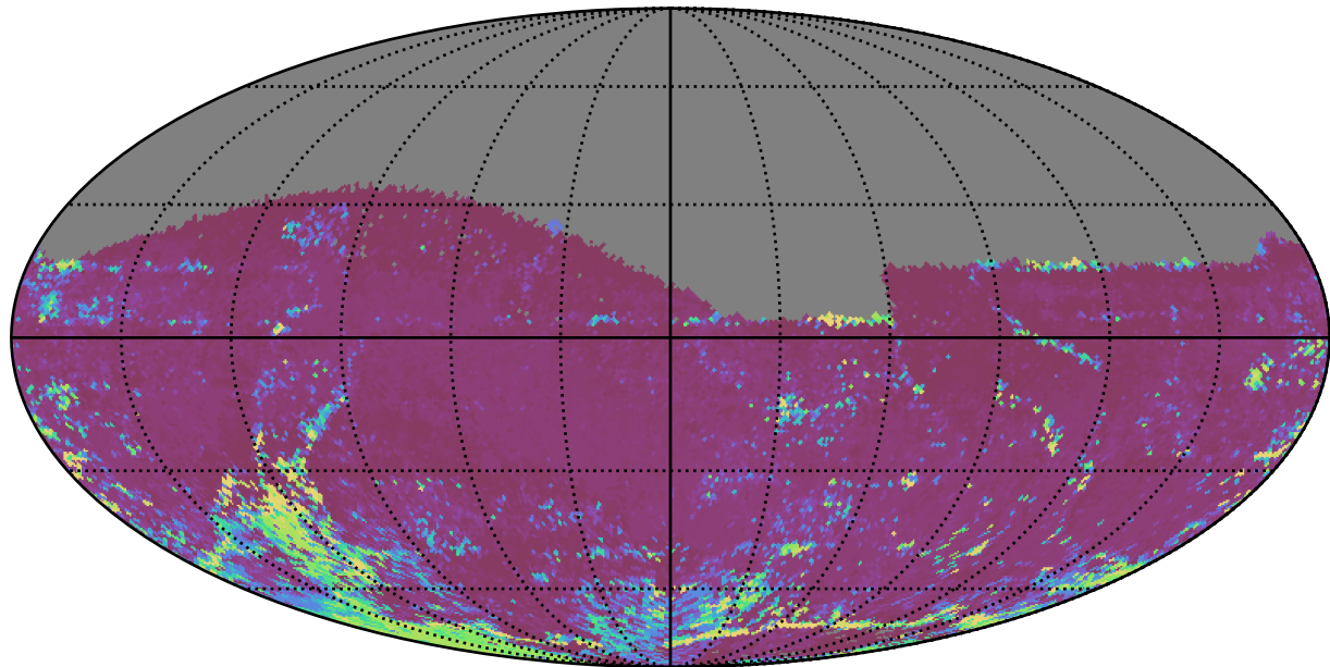
mw_roll_bulge_v3.3_10yrs All sky z band: 75th Percentile Intranight Timespan
