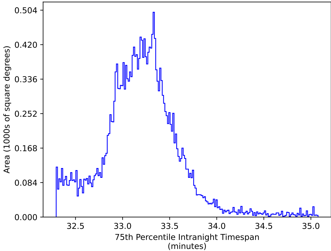
mw_roll_bulge_v3.3_10yrs All sky y band: 75th Percentile Intranight Timespan
