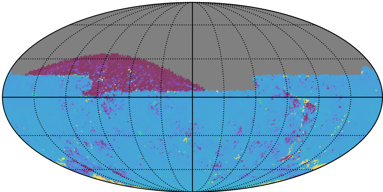
mw_roll_bulge_v3.3_10yrs All sky ug bands: 75th Percentile Intranight Timespan
