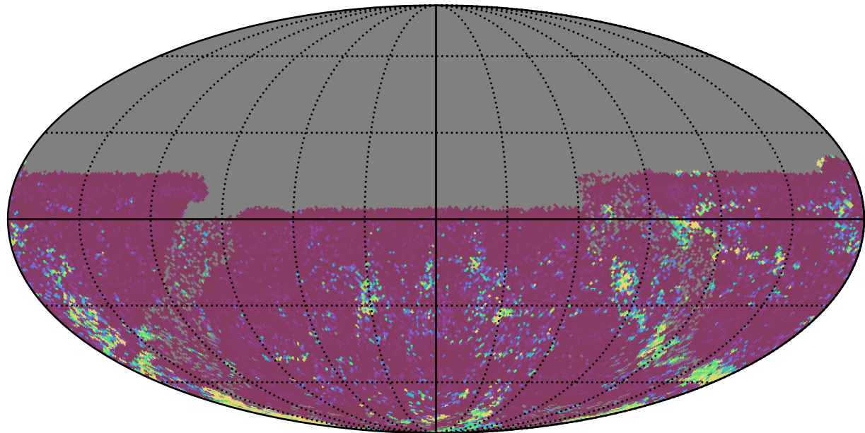
mw_roll_bulge_v3.3_10yrs All sky u band: 75th Percentile Intranight Timespan
