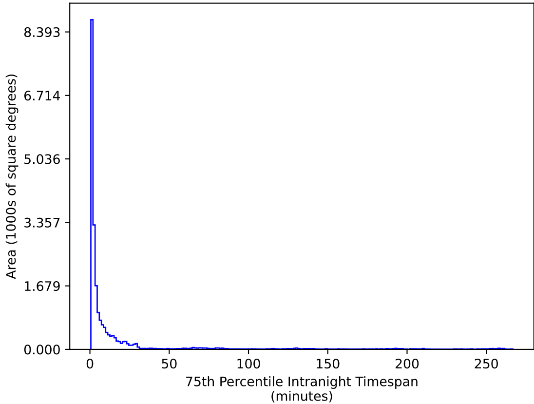
mw_roll_bulge_v3.3_10yrs All sky u band: 75th Percentile Intranight Timespan
