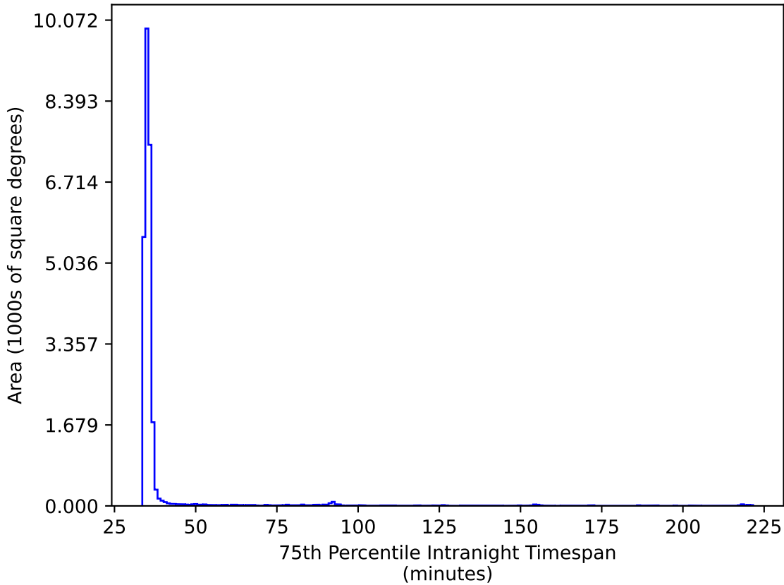
mw_roll_bulge_v3.3_10yrs All sky ri bands: 75th Percentile Intranight Timespan
