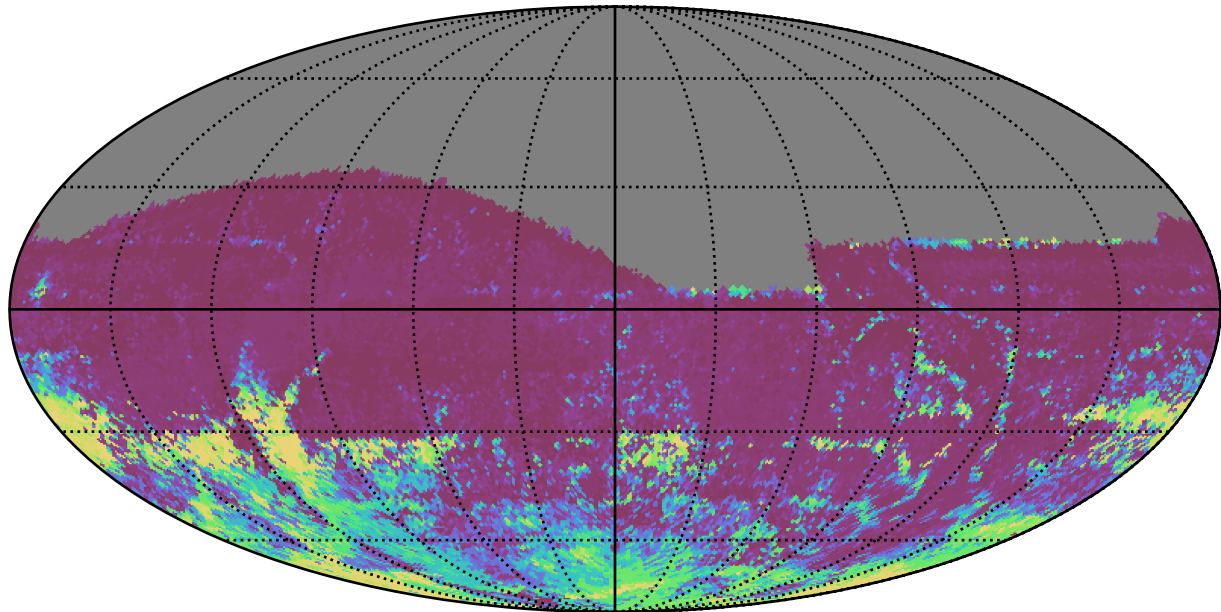
mw_roll_bulge_v3.3_10yrs All sky r band: 75th Percentile Intranight Timespan
