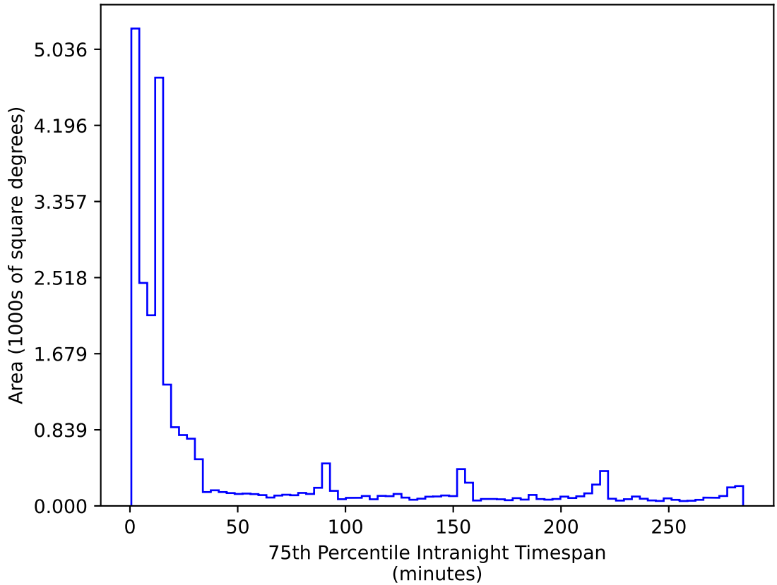
mw_roll_bulge_v3.3_10yrs All sky r band: 75th Percentile Intranight Timespan
