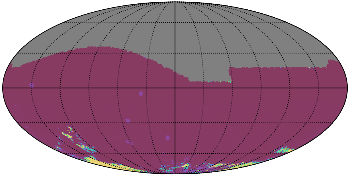
mw_roll_bulge_v3.3_10yrs All sky iz bands: 75th Percentile Intranight Timespan
