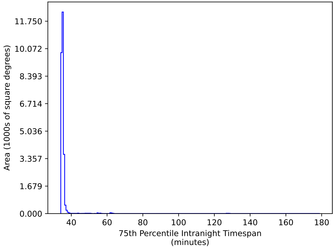
mw_roll_bulge_v3.3_10yrs All sky iz bands: 75th Percentile Intranight Timespan
