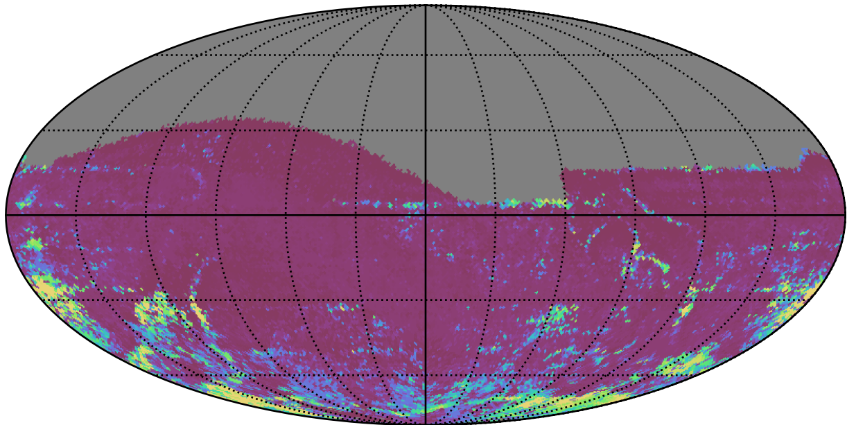
mw_roll_bulge_v3.3_10yrs All sky i band: 75th Percentile Intranight Timespan
