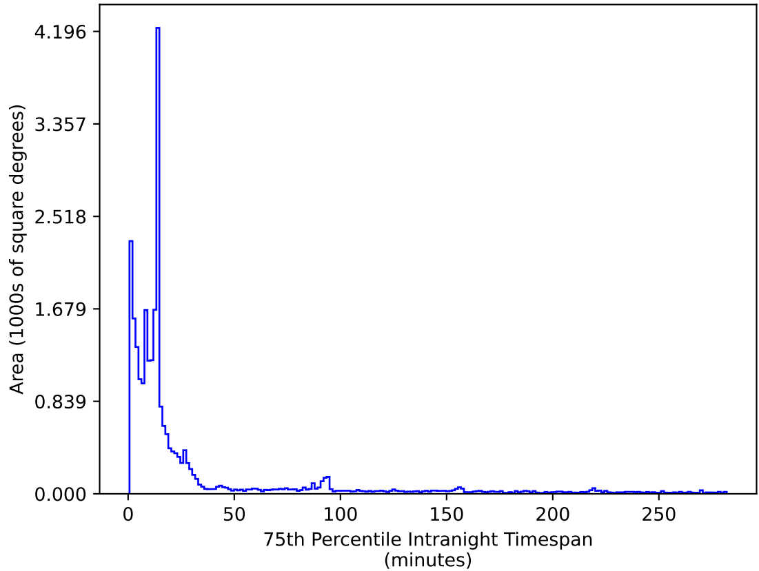
mw_roll_bulge_v3.3_10yrs All sky i band: 75th Percentile Intranight Timespan
