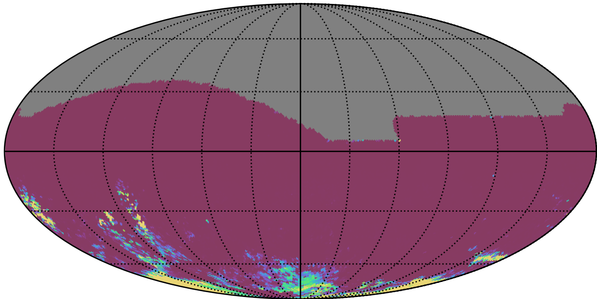
mw_roll_bulge_v3.3_10yrs All sky gr bands: 75th Percentile Intranight Timespan
