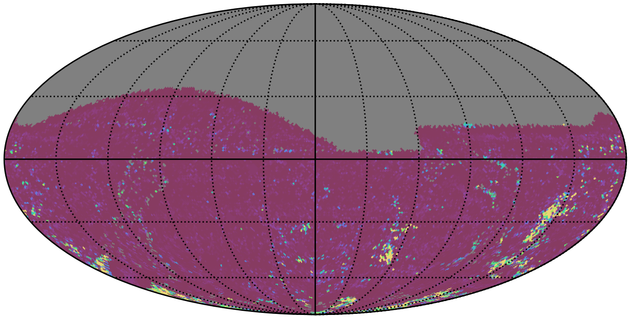
mw_roll_bulge_v3.3_10yrs All sky g band: 75th Percentile Intranight Timespan
