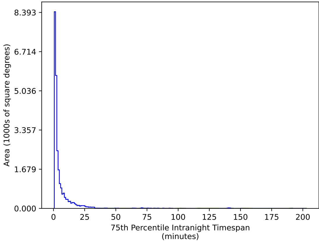
mw_roll_bulge_v3.3_10yrs All sky g band: 75th Percentile Intranight Timespan
