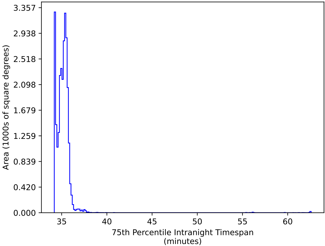
mw_roll_bulge_v3.3_10yrs All sky: 75th Percentile Intranight Timespan
