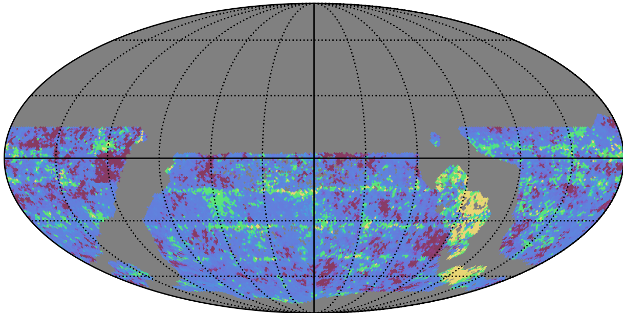
mw_roll_bulge_v3.3_10yrs WFD y band: 20thPercentile Inter-Night Gap
