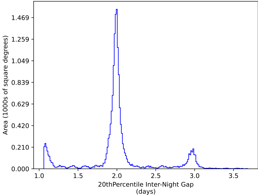
mw_roll_bulge_v3.3_10yrs WFD y band: 20thPercentile Inter-Night Gap
