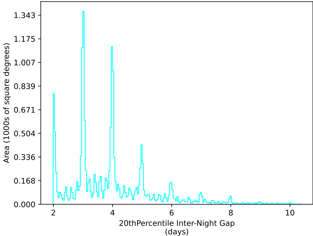
mw_roll_bulge_v3.3_10yrs WFD u band: 20thPercentile Inter-Night Gap
