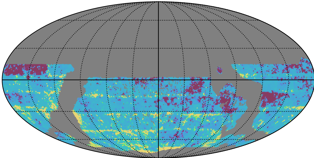
mw_roll_bulge_v3.3_10yrs WFD r band: 20thPercentile Inter-Night Gap
