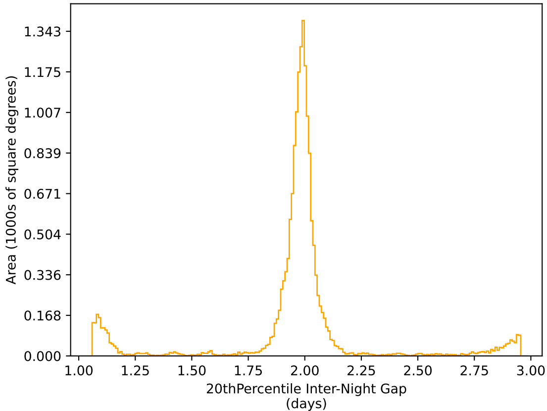
mw_roll_bulge_v3.3_10yrs WFD r band: 20thPercentile Inter-Night Gap
