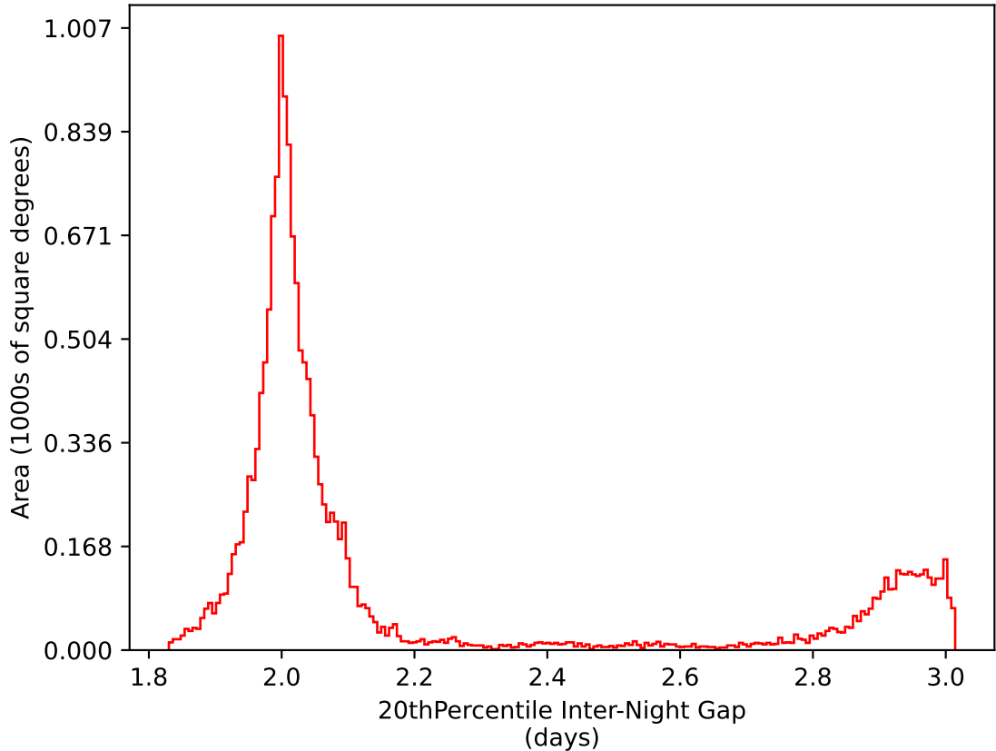
mw_roll_bulge_v3.3_10yrs WFD i band: 20thPercentile Inter-Night Gap
