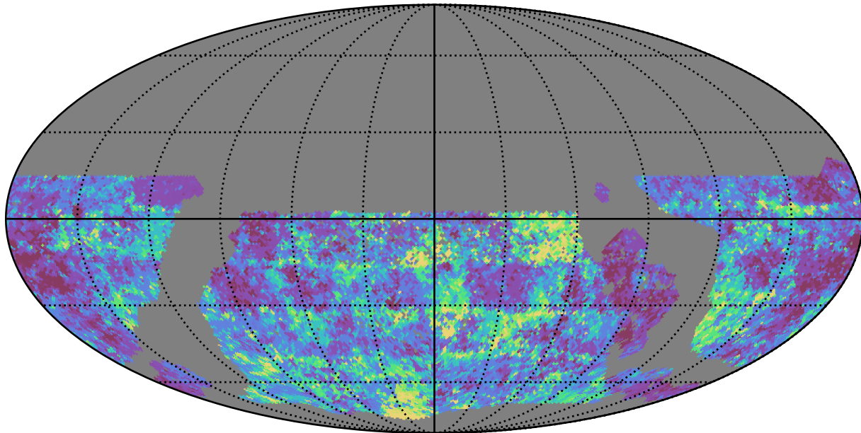
mw_roll_bulge_v3.3_10yrs WFD g band: 20thPercentile Inter-Night Gap
