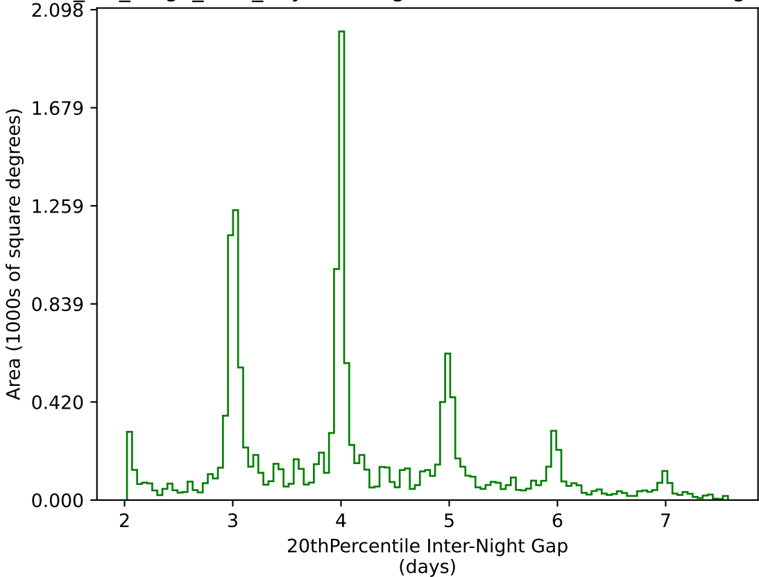
mw_roll_bulge_v3.3_10yrs WFD g band: 20thPercentile Inter-Night Gap
